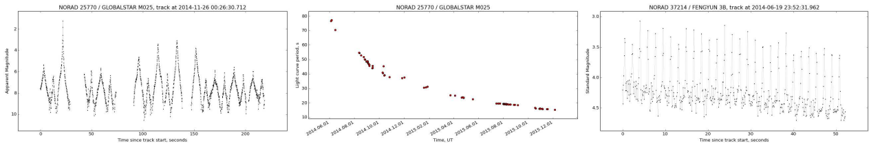
Fig. 6. Light curve of an freely rotating inactive satellite detected by Mini-MegaTORTORA (left), its period evolution over time due to interaction with atmosphere and residual technological processes (center) and the rapid variability of an active satellite due to stabilized antenna rotation with 1.8 s period (right).
