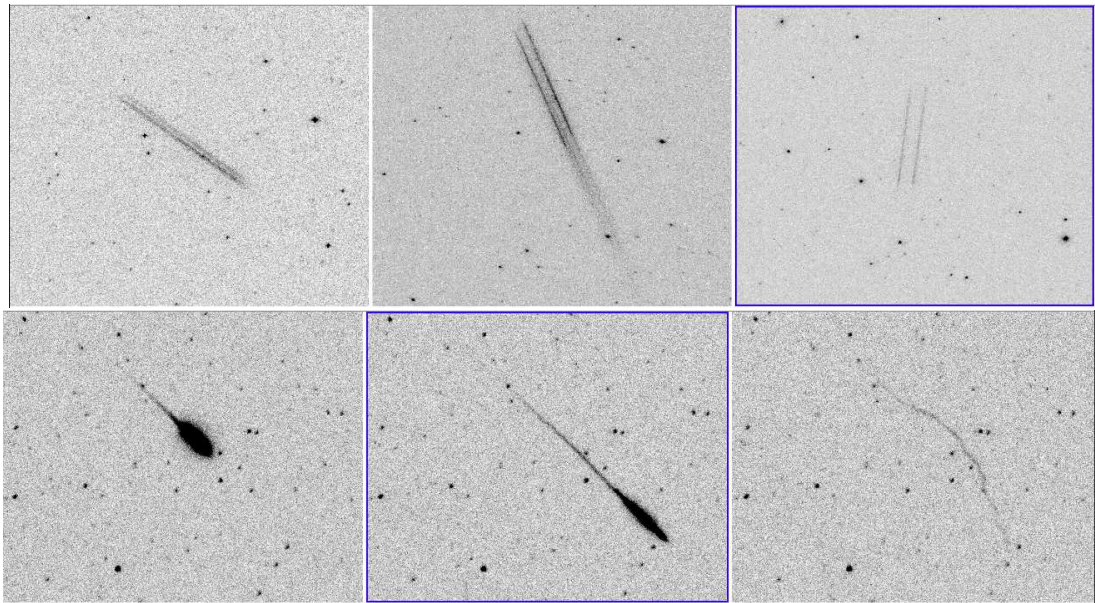
Fig. 4. Example of multi-particle meteor trails (top) and the complex temporal evolution of a bolide trail in the atmosphere (bottom).
