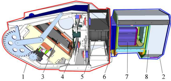
Fig. 1. Schematic view of a MMT channel. 1 – celostate unit, 2 – camera unit, 3 – celostate mirror which can rotate for \sim 10 degrees around two axes, 4 – installable color and polarimetric filters, 5 – Canon EF85/1.2 objective, 6 – optical corrector, 7 – Andor Neo sCMOS detector, 8 – conditioner to keep stable environmental conditions inside the channel.
