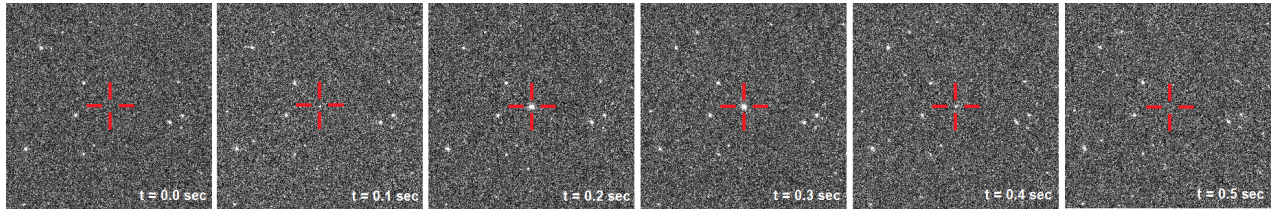
Fig. 7. Rapid optical flash detected by MMT, with duration less than 0.5 s and peak brightness reaching \sim 6.5^m . The flash coincides with the high-altitude passage of MOLNIYA satellite.
