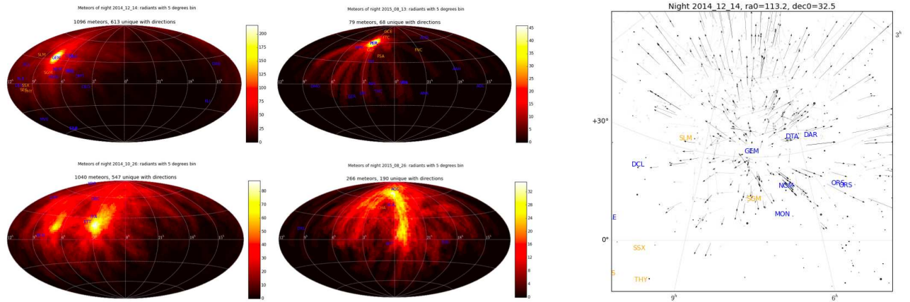
Fig. 3. Density of intersections of meteor trails from the night corresponding to the peak of 2014 Geminids (left) and meteor trails corresponding to the Geminids shower in gnomonic projection (right).
